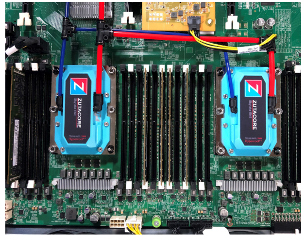
ZutaCore direct-on-chip evaporative cooling for Intel Skylake on Open19 server
